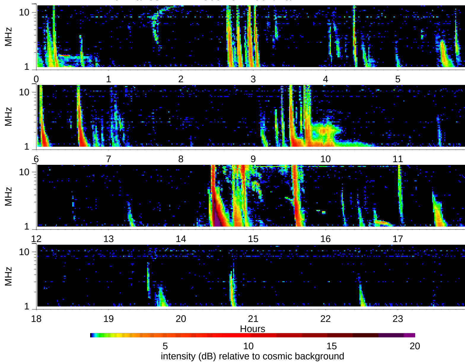
Wind Waves RAD2 receiver: 2002/10/14
