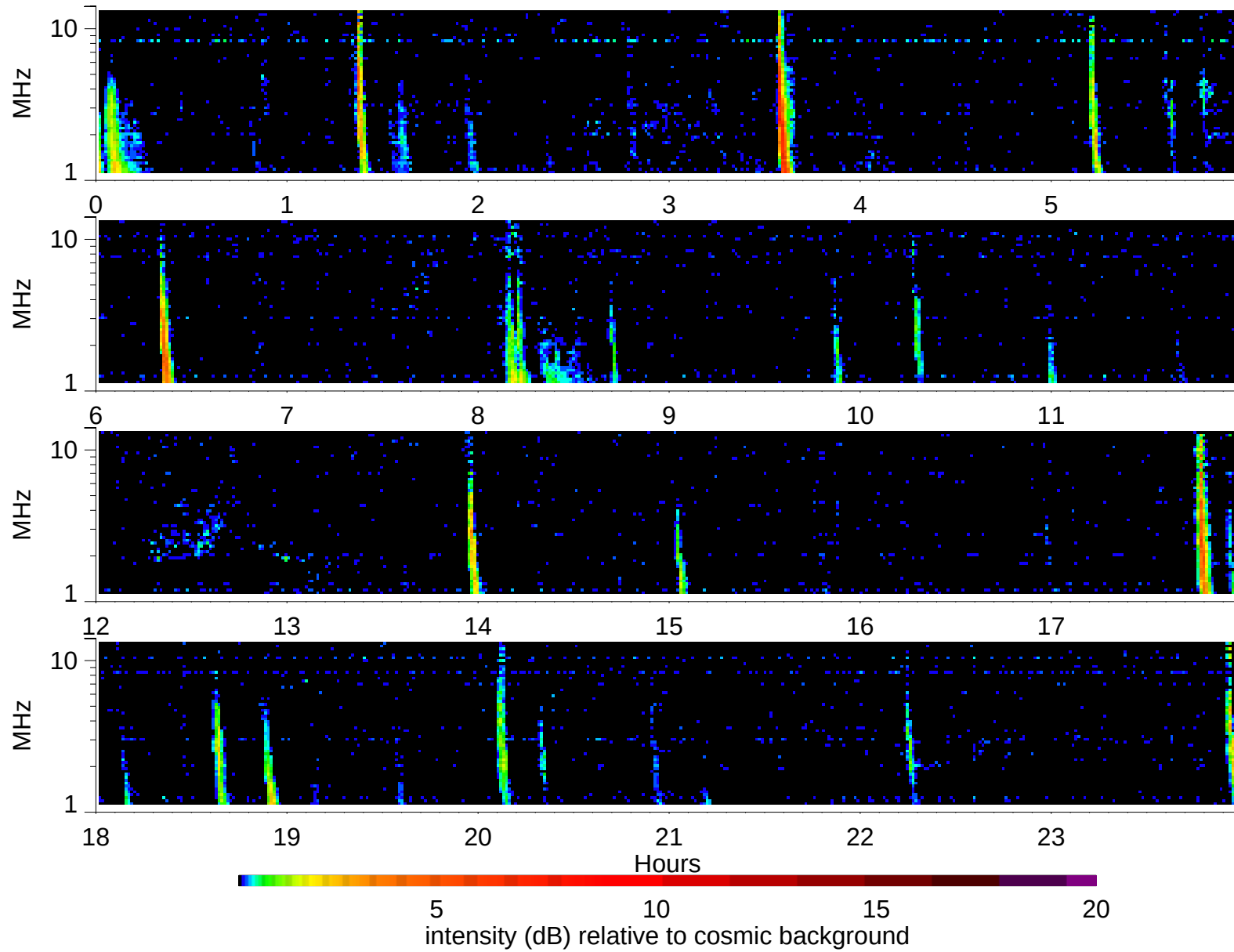
Wind Waves RAD2 receiver: 2002/10/18
