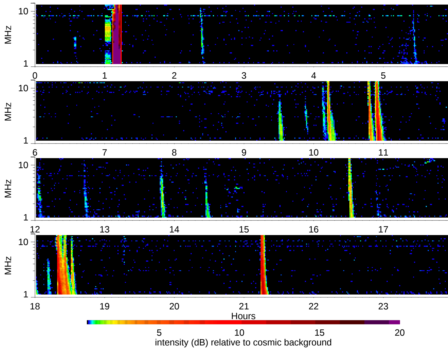
Wind Waves RAD2 receiver: 2002/10/19
