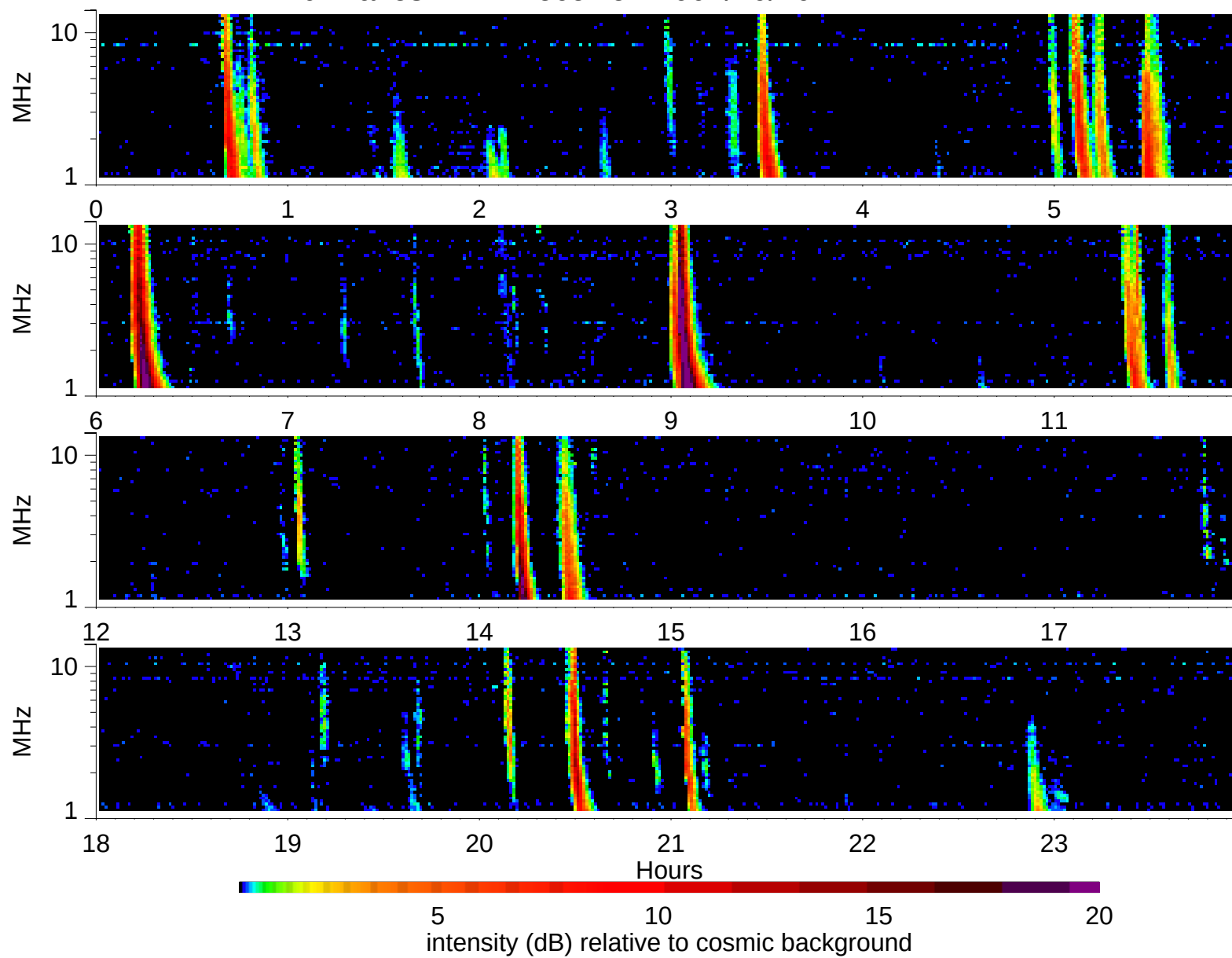
Wind Waves RAD2 receiver: 2002/10/20
