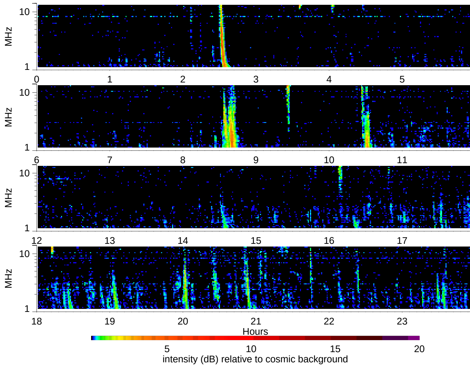
Wind Waves RAD2 receiver: 2002/10/22
