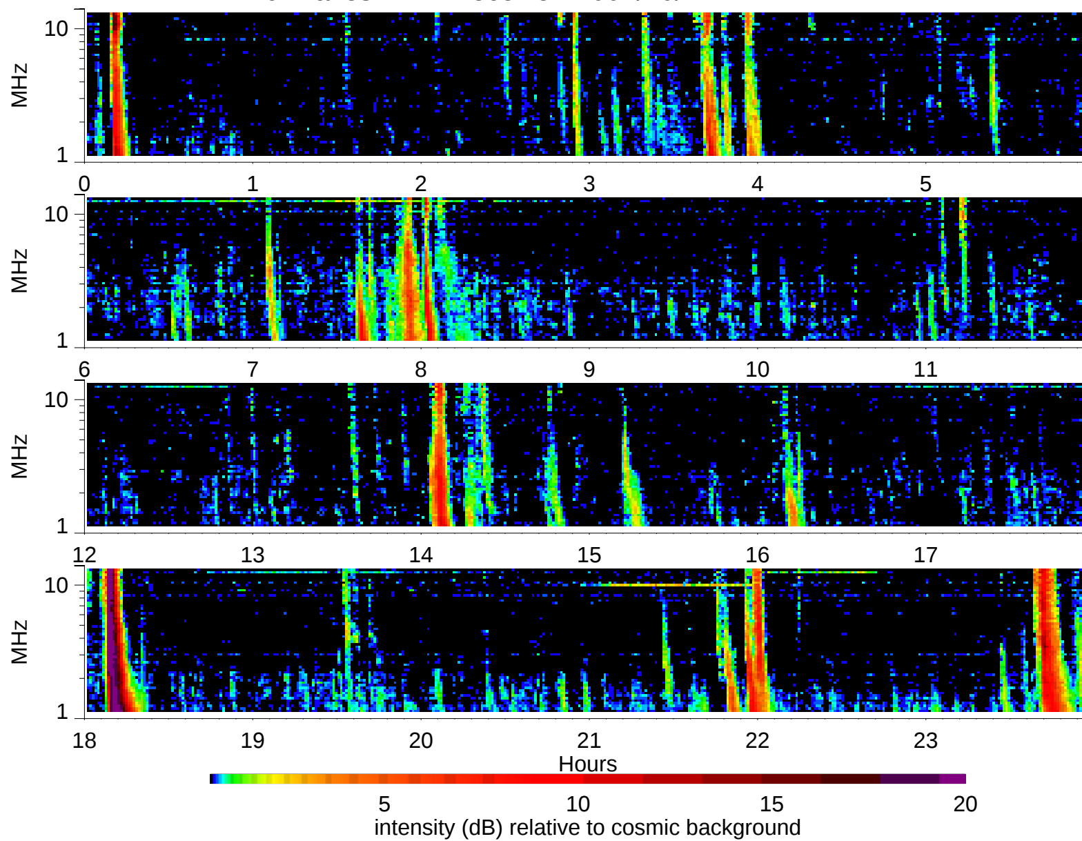
Wind Waves RAD2 receiver: 2002/10/24
