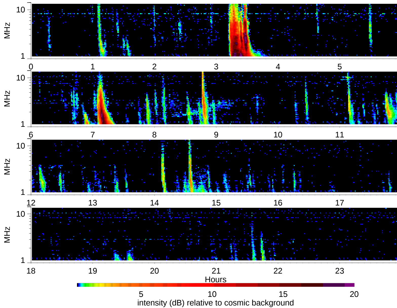
Wind Waves RAD2 receiver: 2002/10/26
