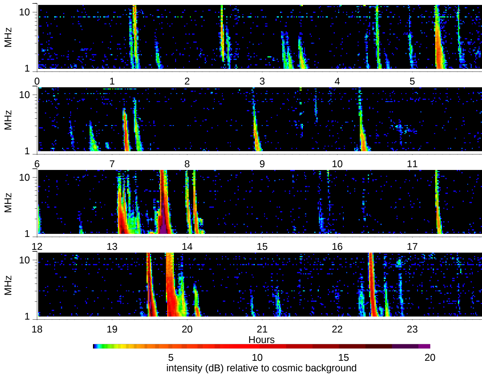
Wind Waves RAD2 receiver: 2002/10/28
