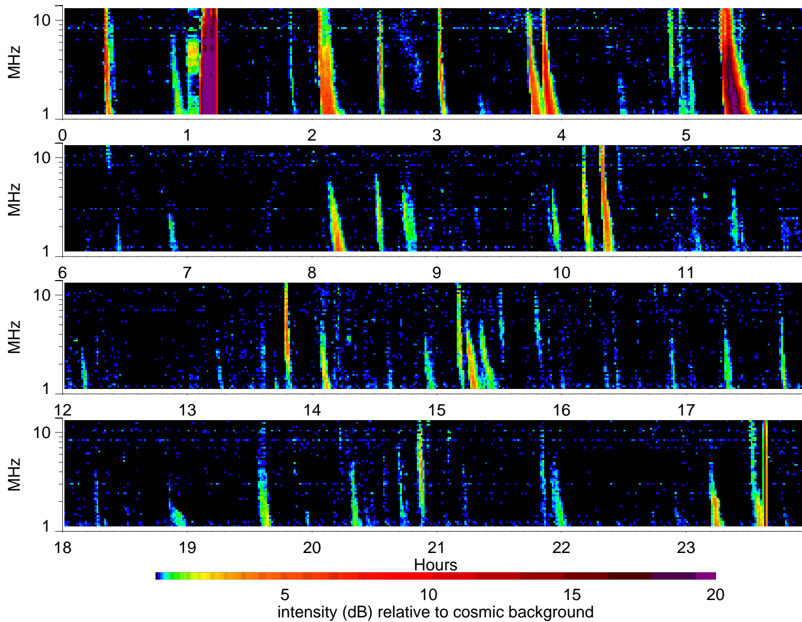
Wind Waves RAD2 receiver: 2002/10/29
