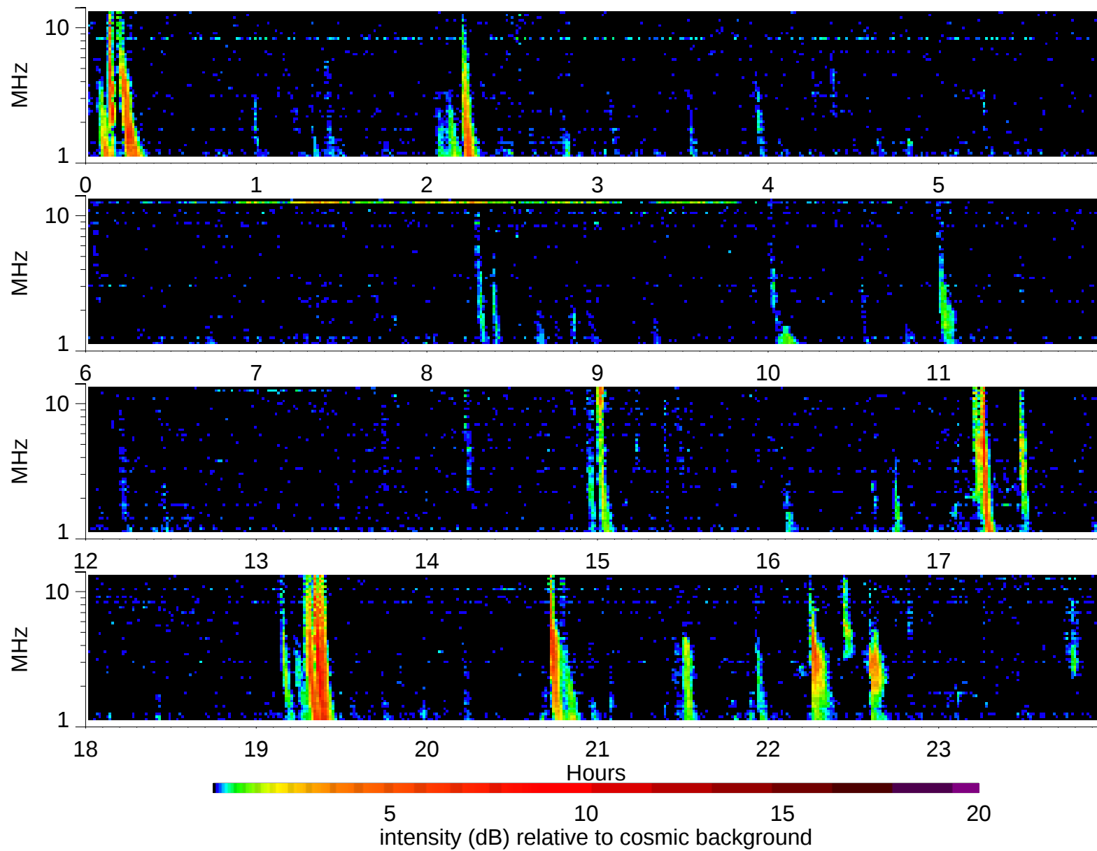
Wind Waves RAD2 receiver: 2002/10/30
