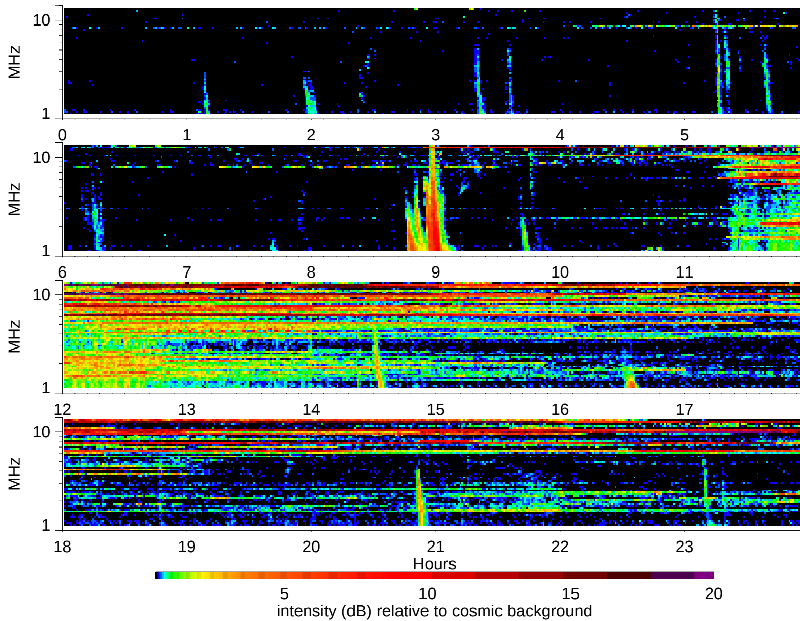
Wind Waves RAD2 receiver: 2002/11/1
