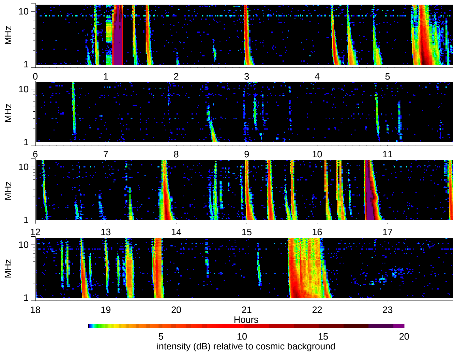
Wind Waves RAD2 receiver: 2002/11/6
