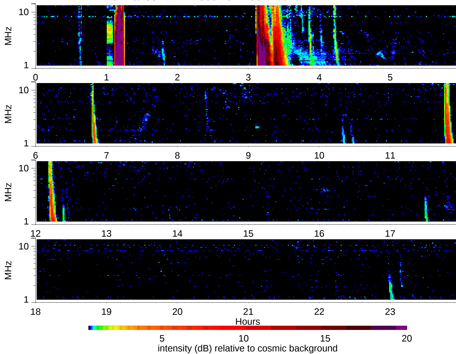
Wind Waves RAD2 receiver: 2002/11/10
