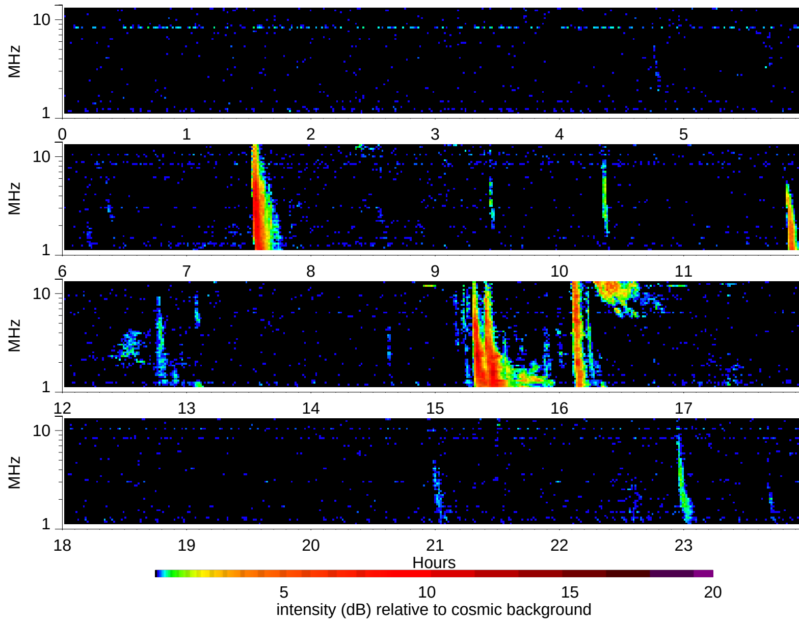
Wind Waves RAD2 receiver: 2002/11/11
