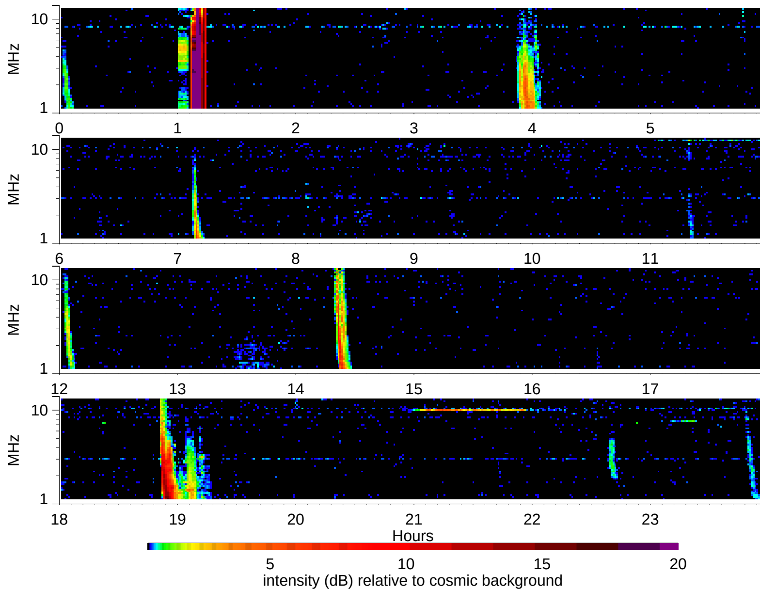
Wind Waves RAD2 receiver: 2002/11/12
