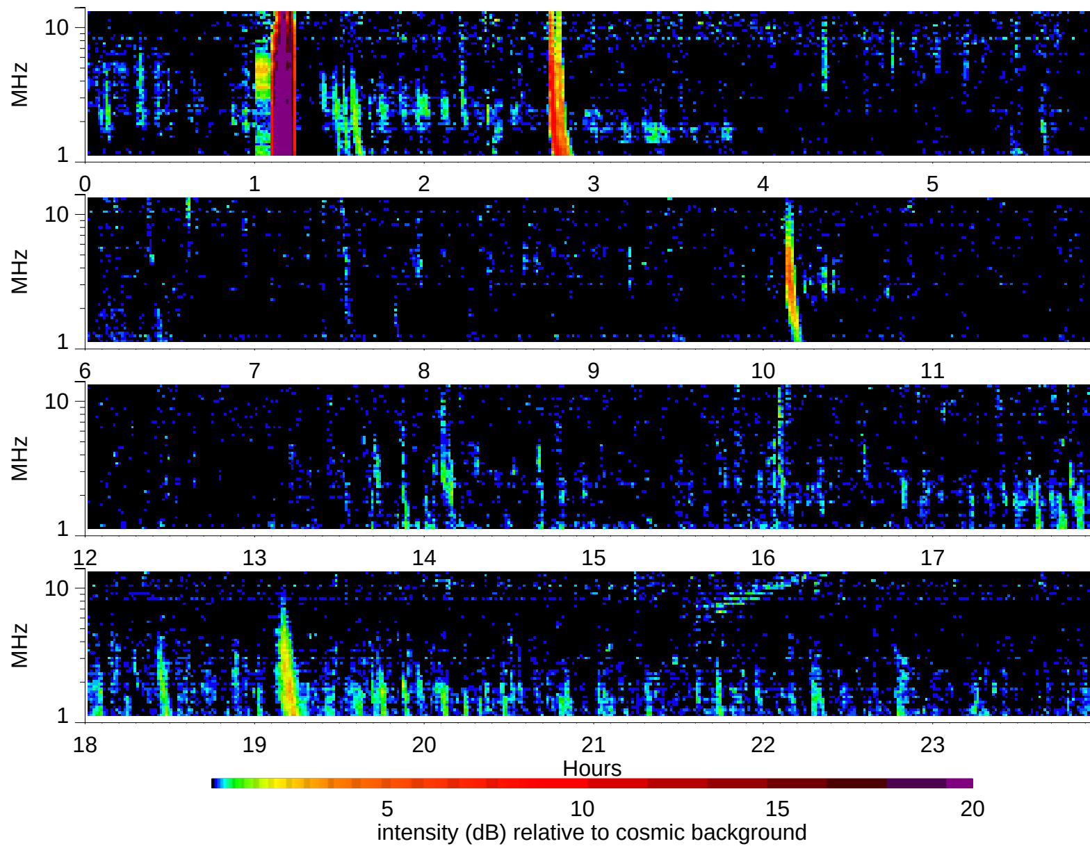
Wind Waves RAD2 receiver: 2002/11/14
