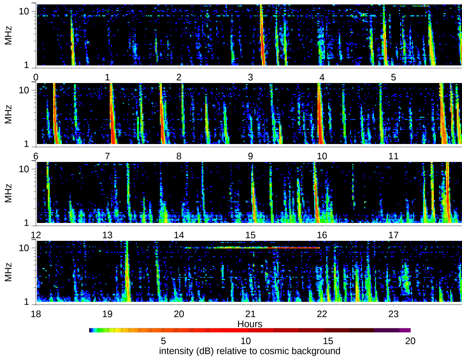
Wind Waves RAD2 receiver: 2002/11/19
