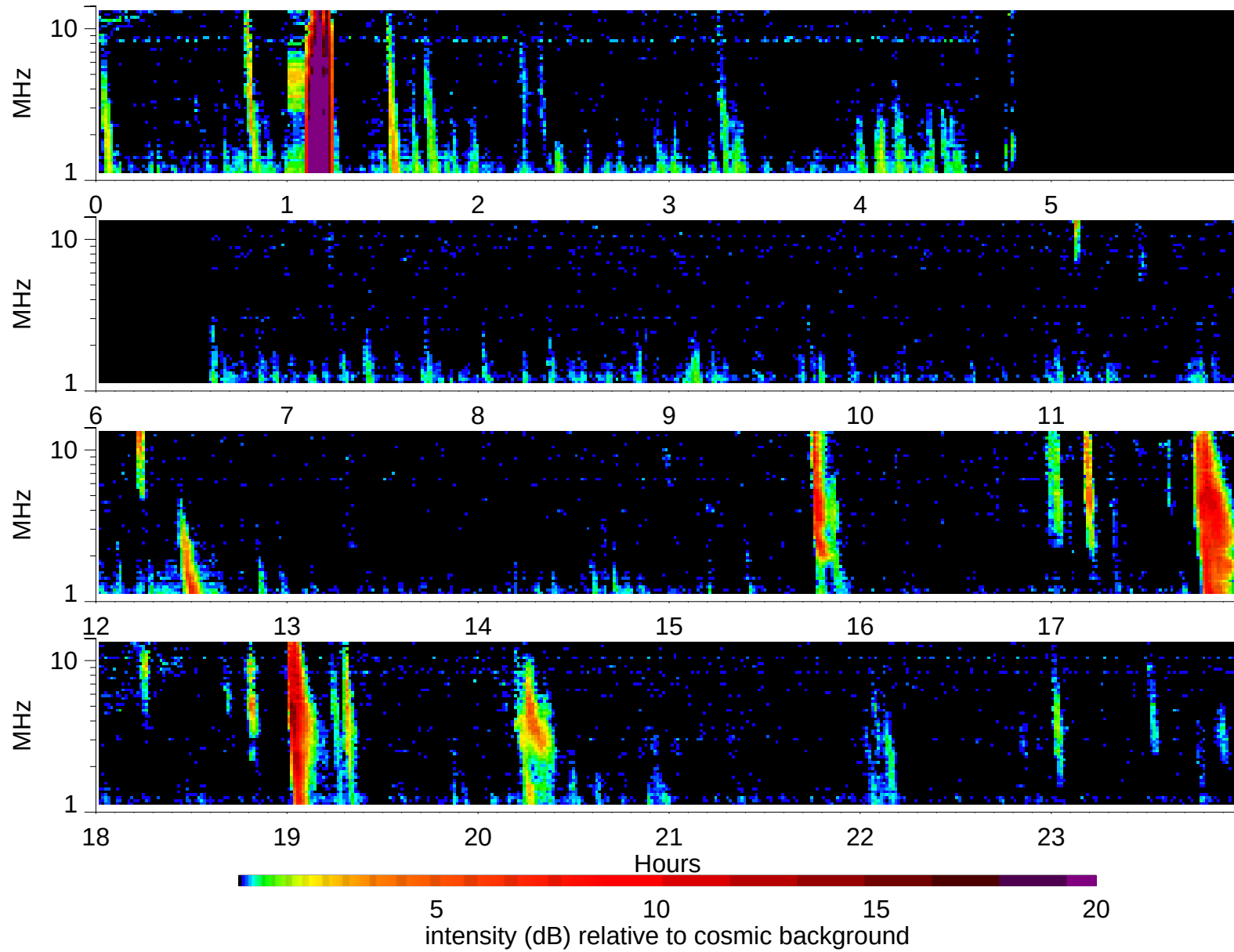
Wind Waves RAD2 receiver: 2002/11/22
