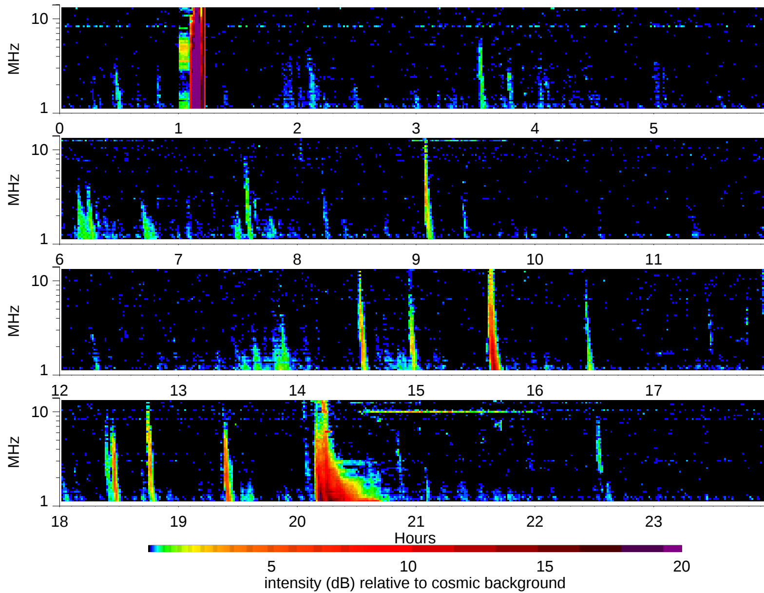
Wind Waves RAD2 receiver: 2002/11/24
