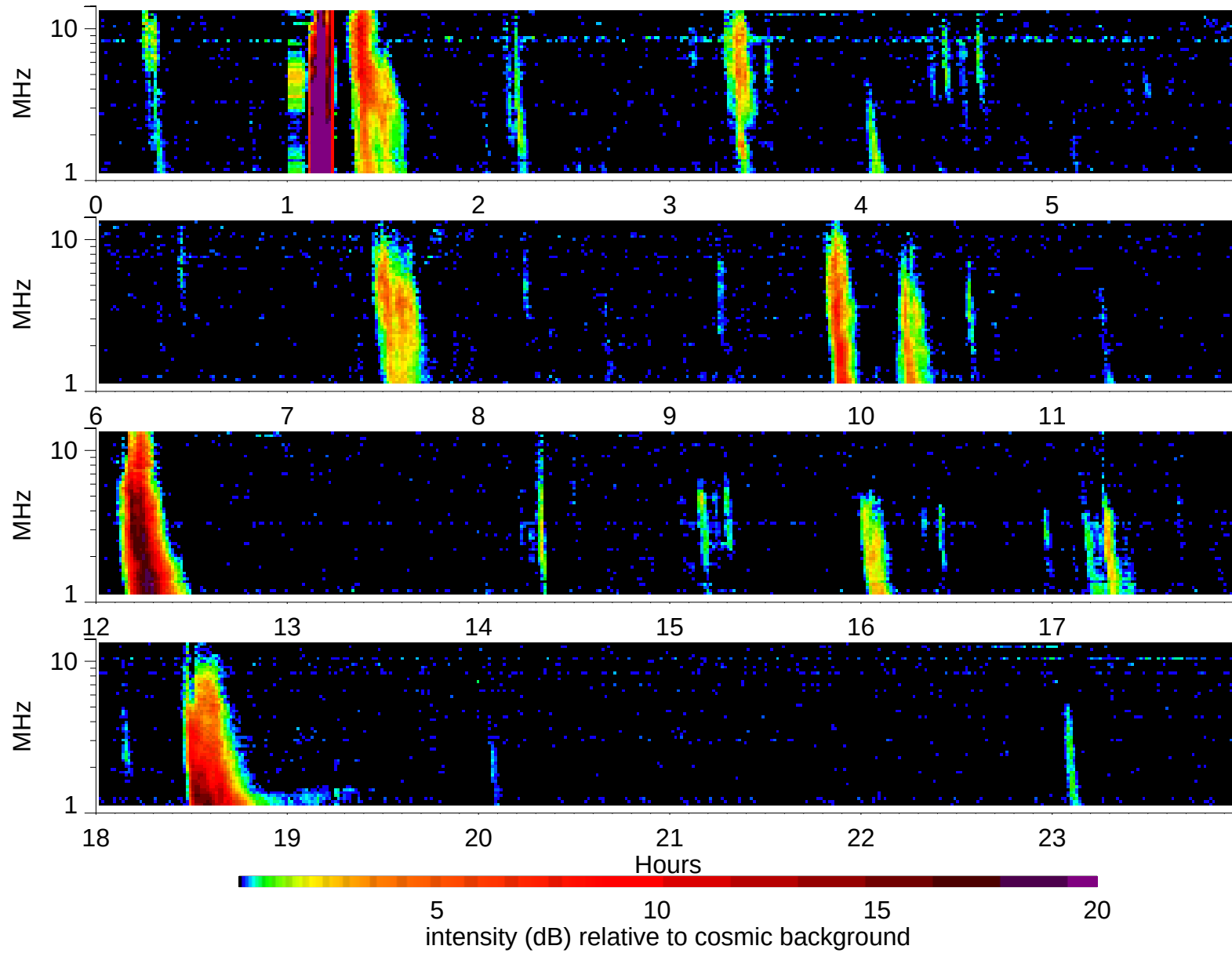
Wind Waves RAD2 receiver: 2002/11/26
