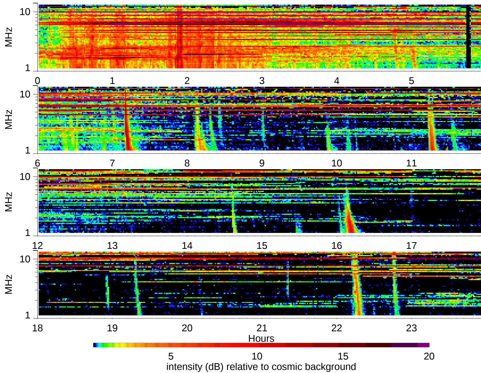
Wind Waves RAD2 receiver: 2002/11/28
