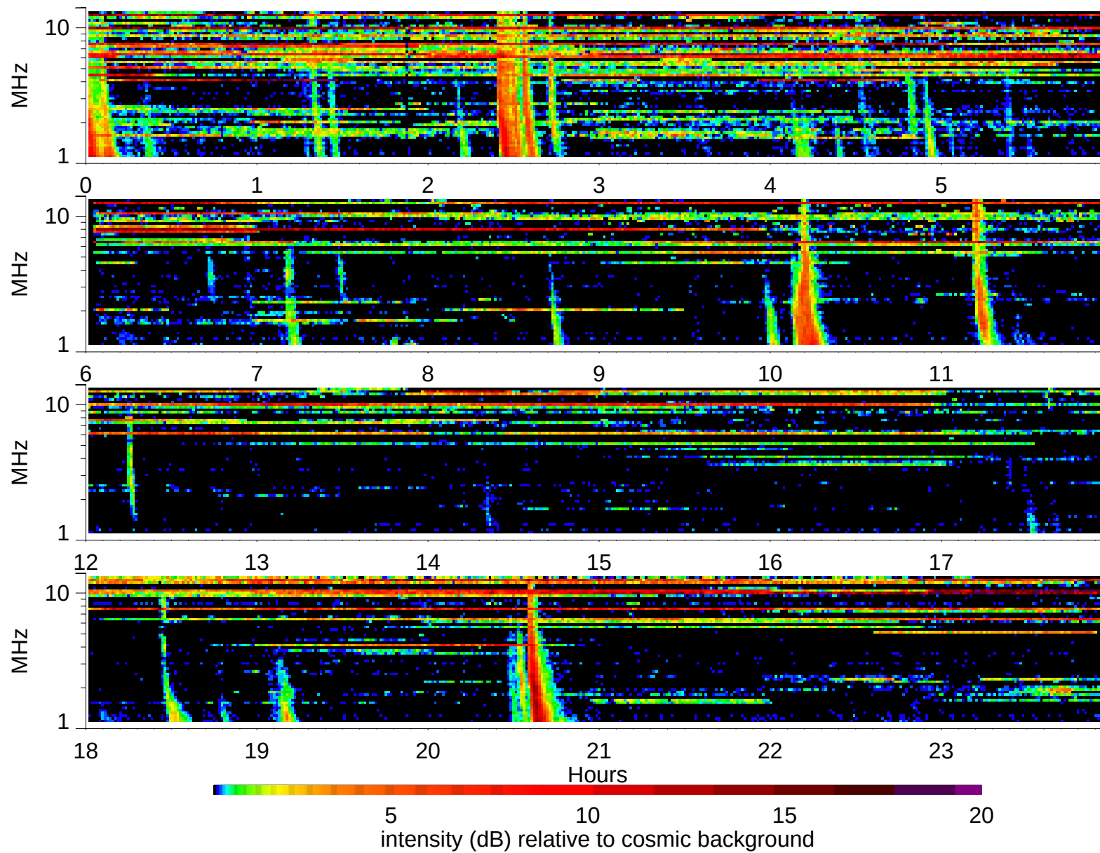
Wind Waves RAD2 receiver: 2002/11/29
