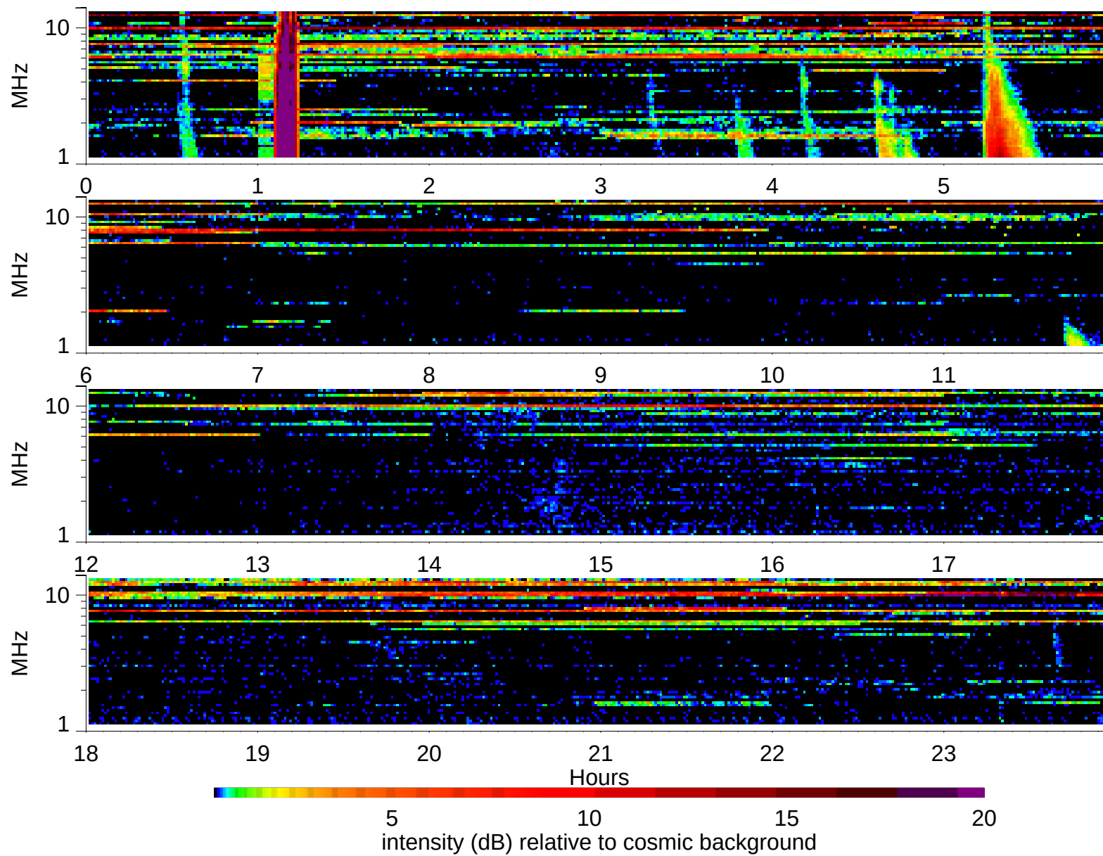
Wind Waves RAD2 receiver: 2002/11/30
