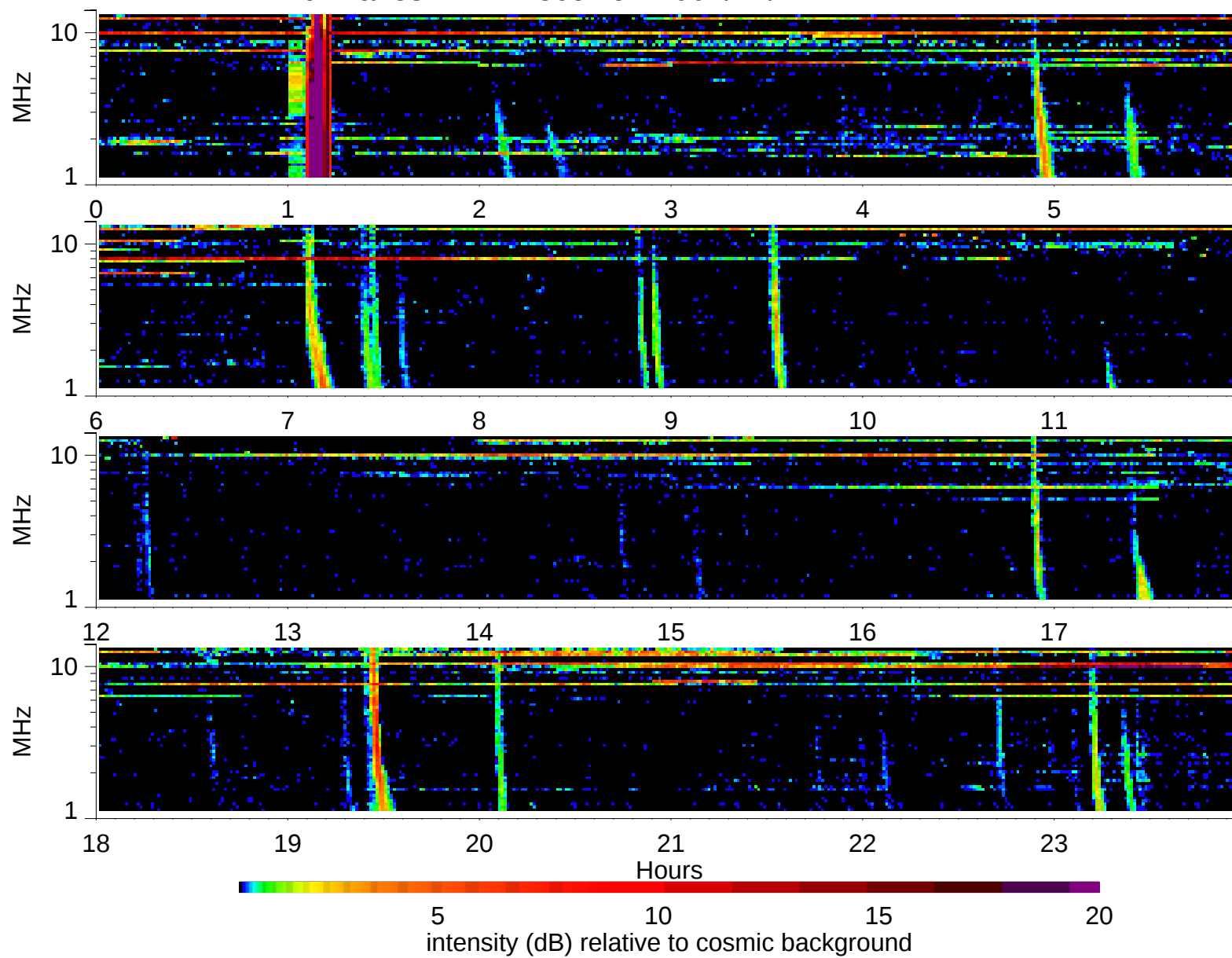
Wind Waves RAD2 receiver: 2002/12/2
