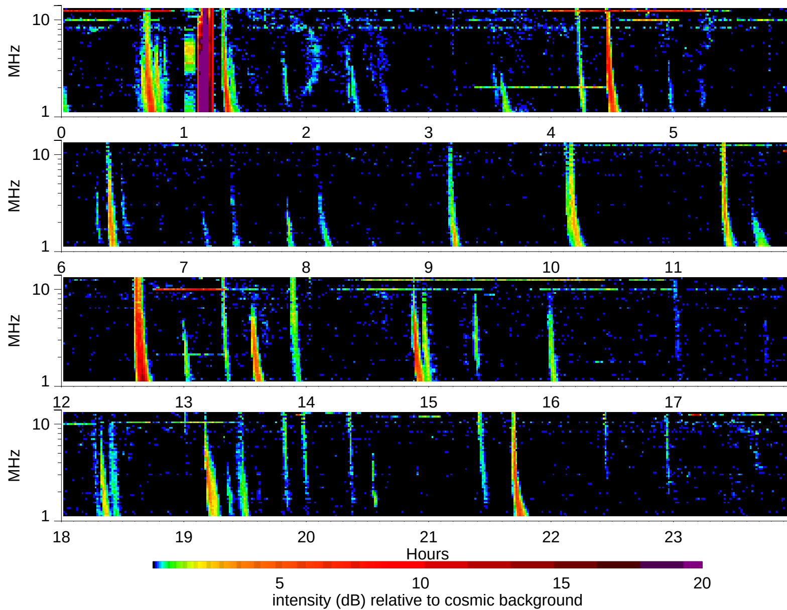
Wind Waves RAD2 receiver: 2002/12/12
