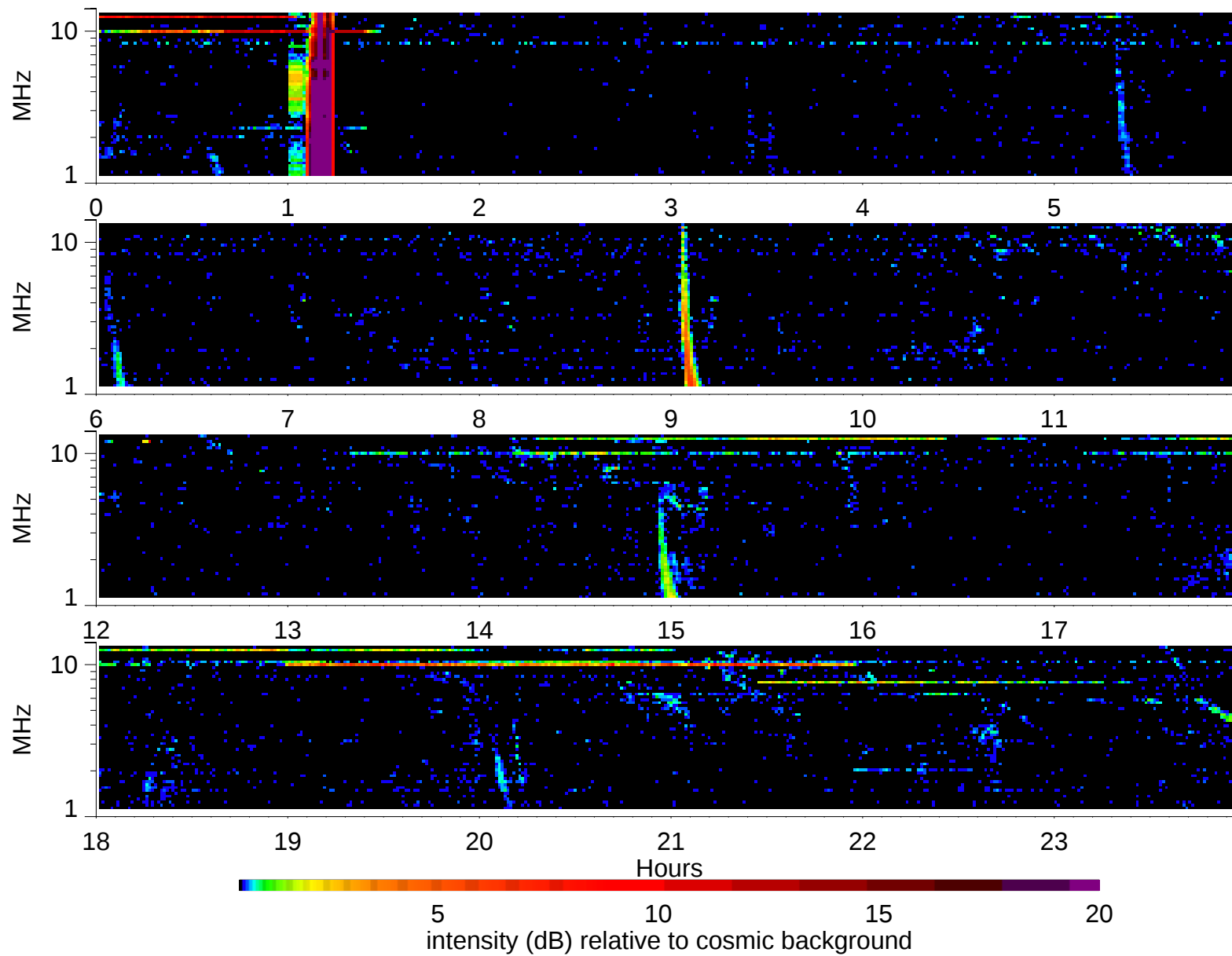
Wind Waves RAD2 receiver: 2002/12/14
