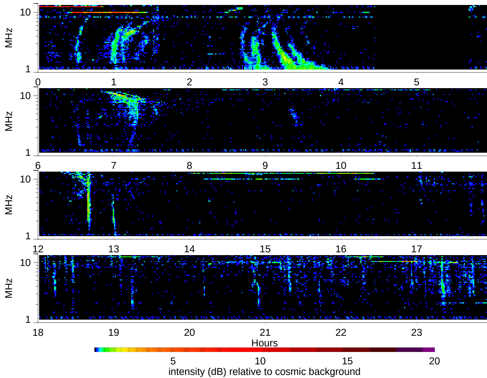
Wind Waves RAD2 receiver: 2002/12/17
