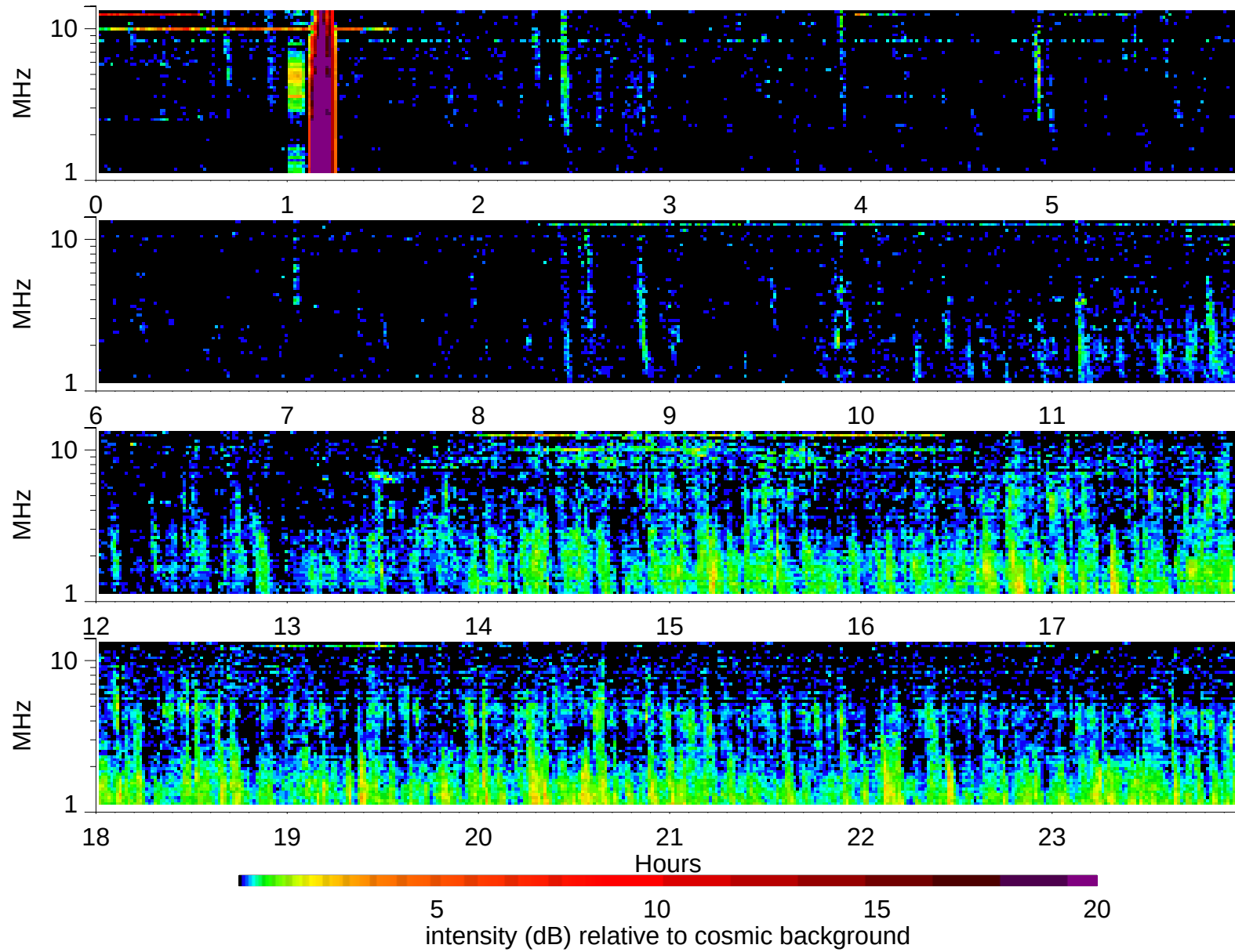
Wind Waves RAD2 receiver: 2002/12/18
