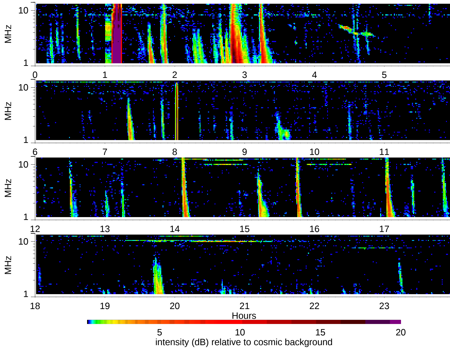
Wind Waves RAD2 receiver: 2002/12/22
