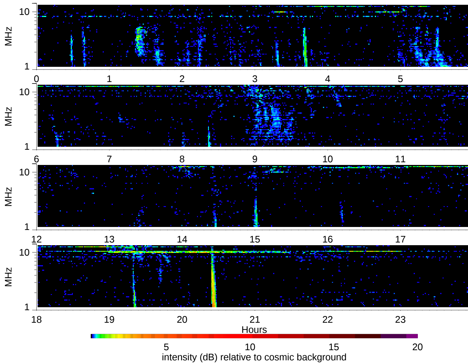
Wind Waves RAD2 receiver: 2002/12/25
