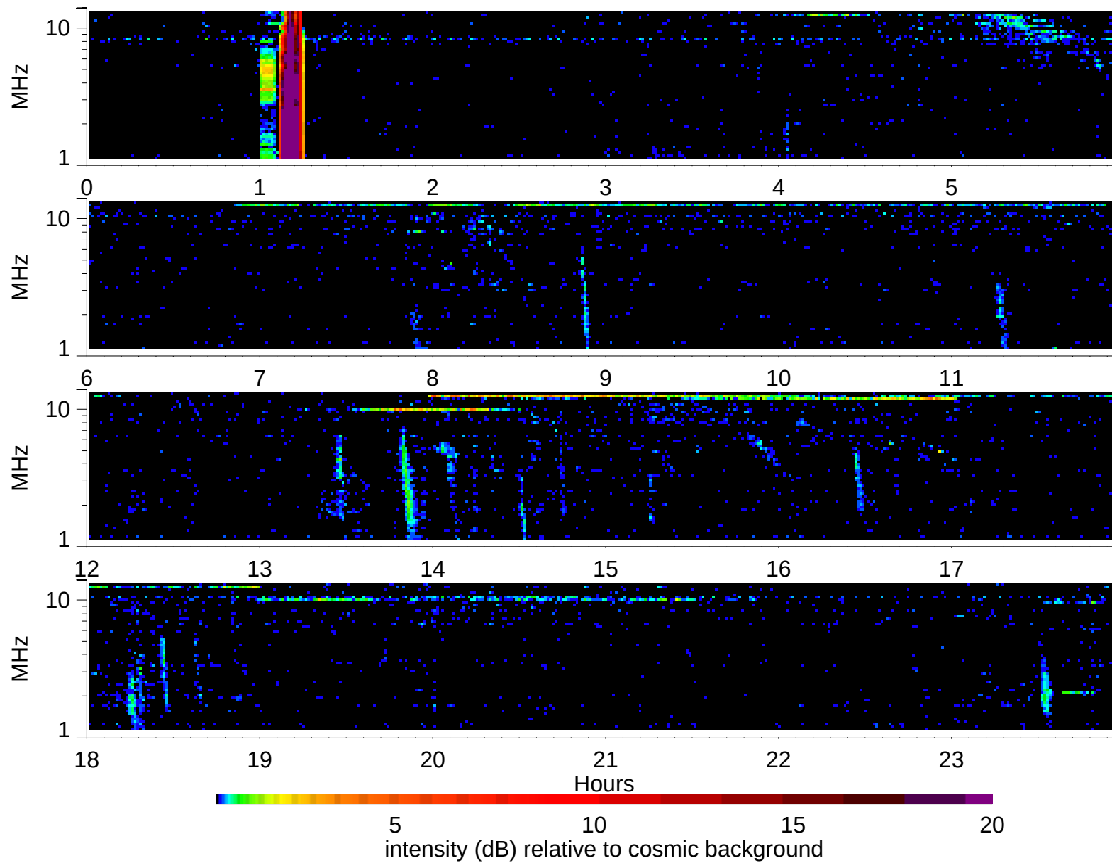
Wind Waves RAD2 receiver: 2002/12/26
