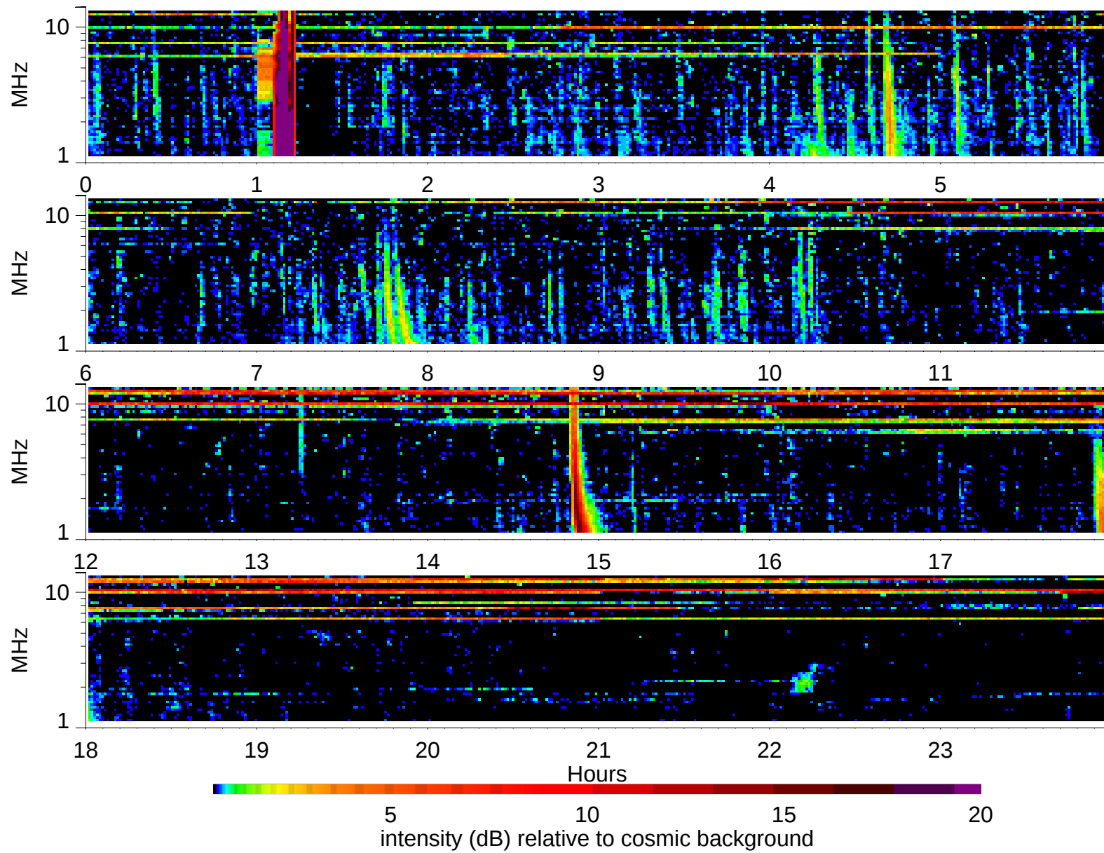
Wind Waves RAD2 receiver: 2004/3/20
