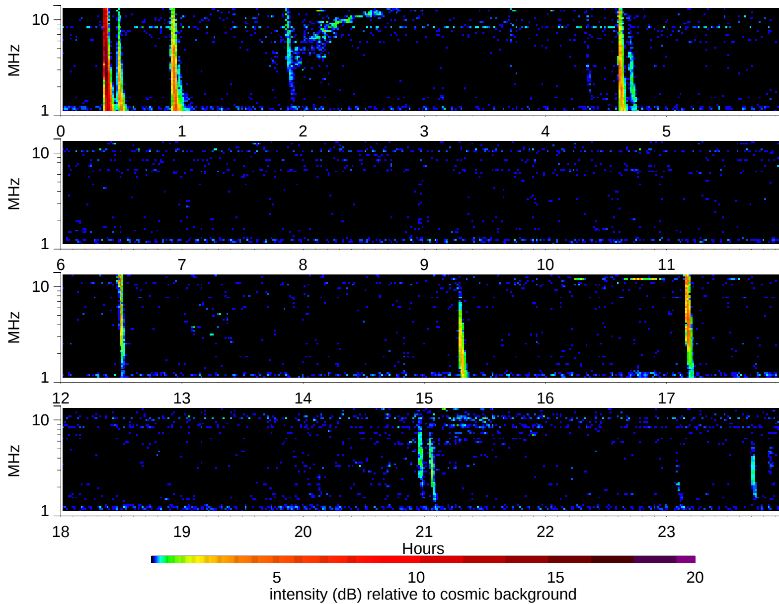
Wind Waves RAD2 receiver: 2005/1/21
