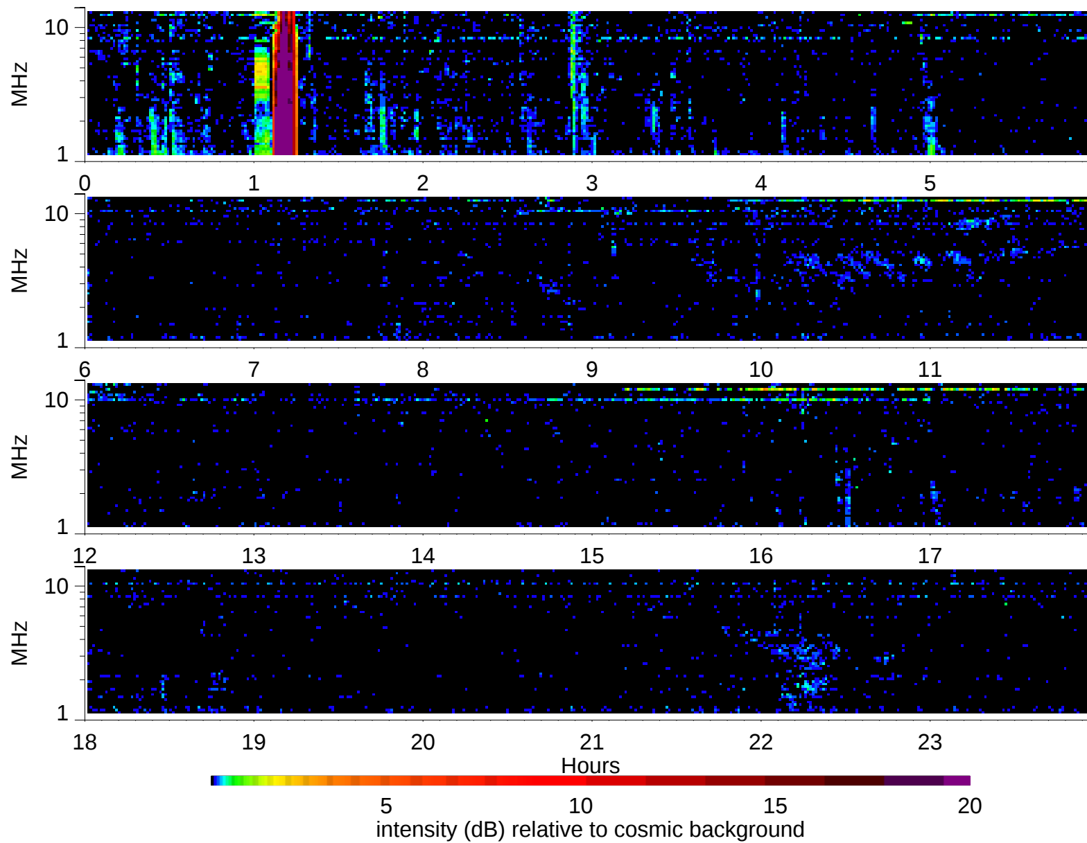
Wind Waves RAD2 receiver: 2005/1/30
