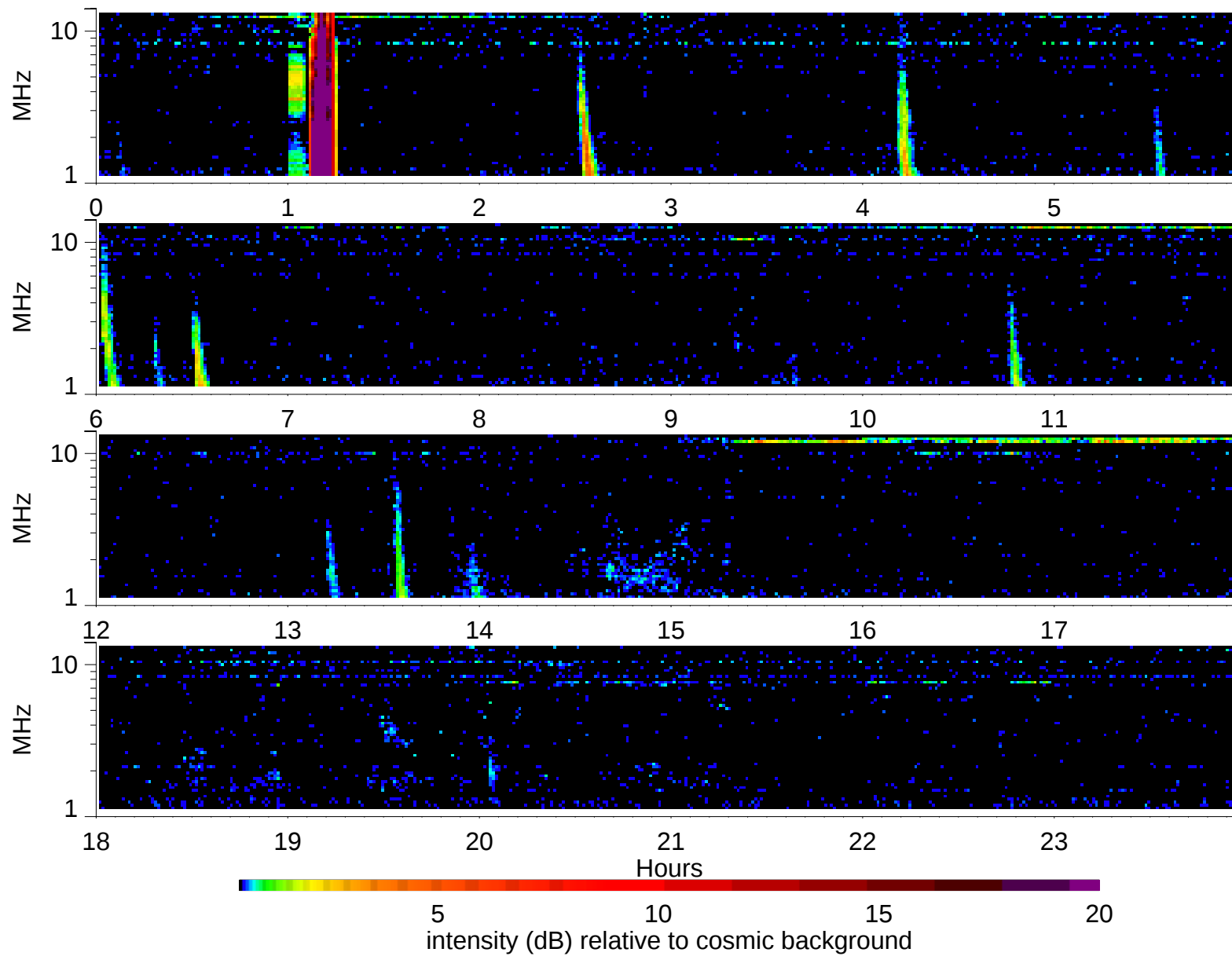
Wind Waves RAD2 receiver: 2005/2/7
