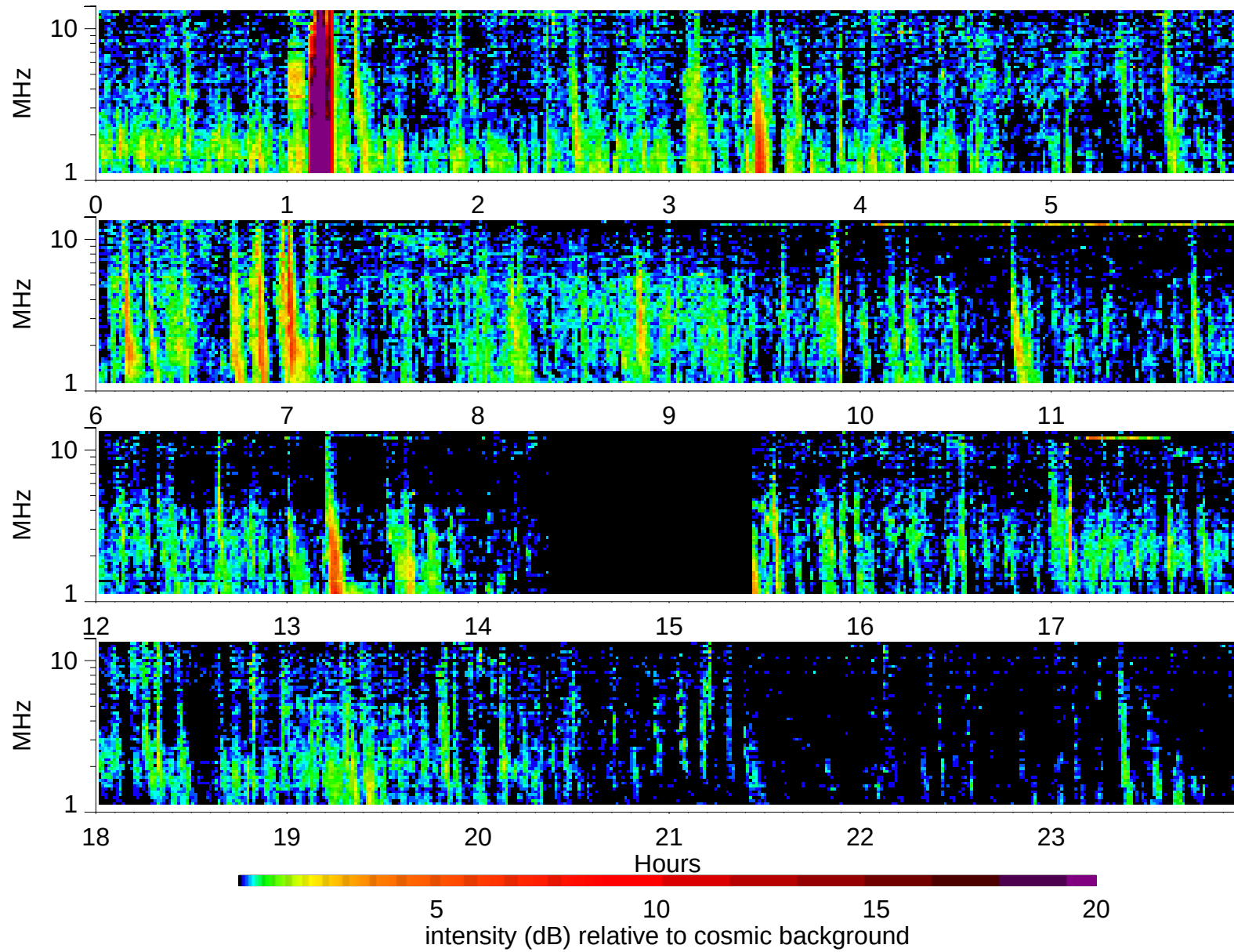
Wind Waves RAD2 receiver: 2005/2/15
