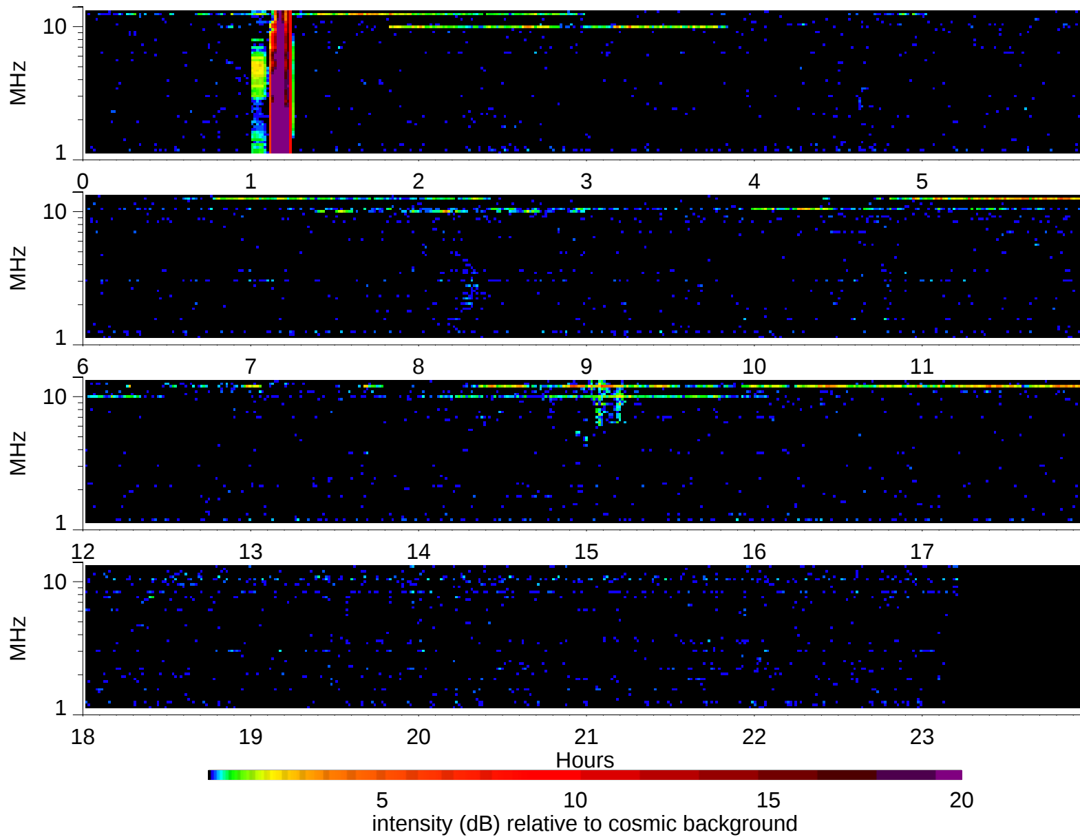
Wind Waves RAD2 receiver: 2005/4/2
