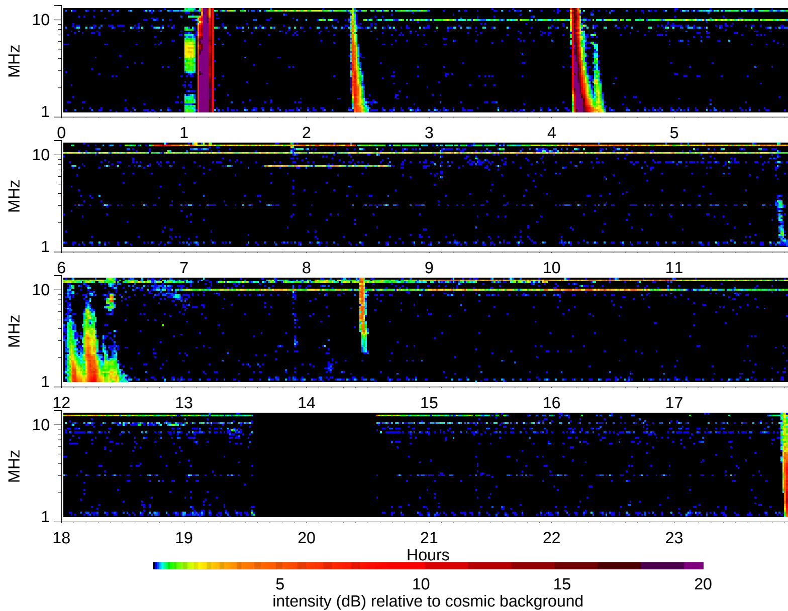
Wind Waves RAD2 receiver: 2005/6/3
