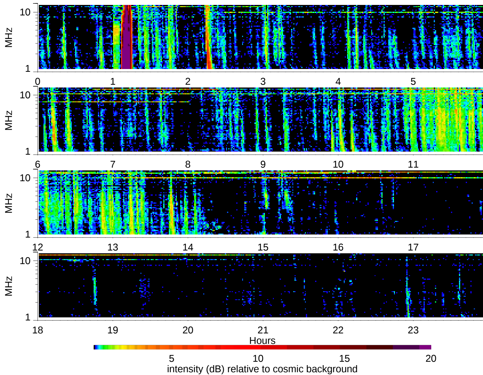
Wind Waves RAD2 receiver: 2005/6/9
