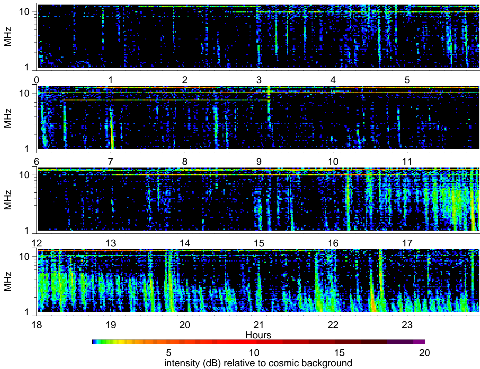
Wind Waves RAD2 receiver: 2005/6/10
