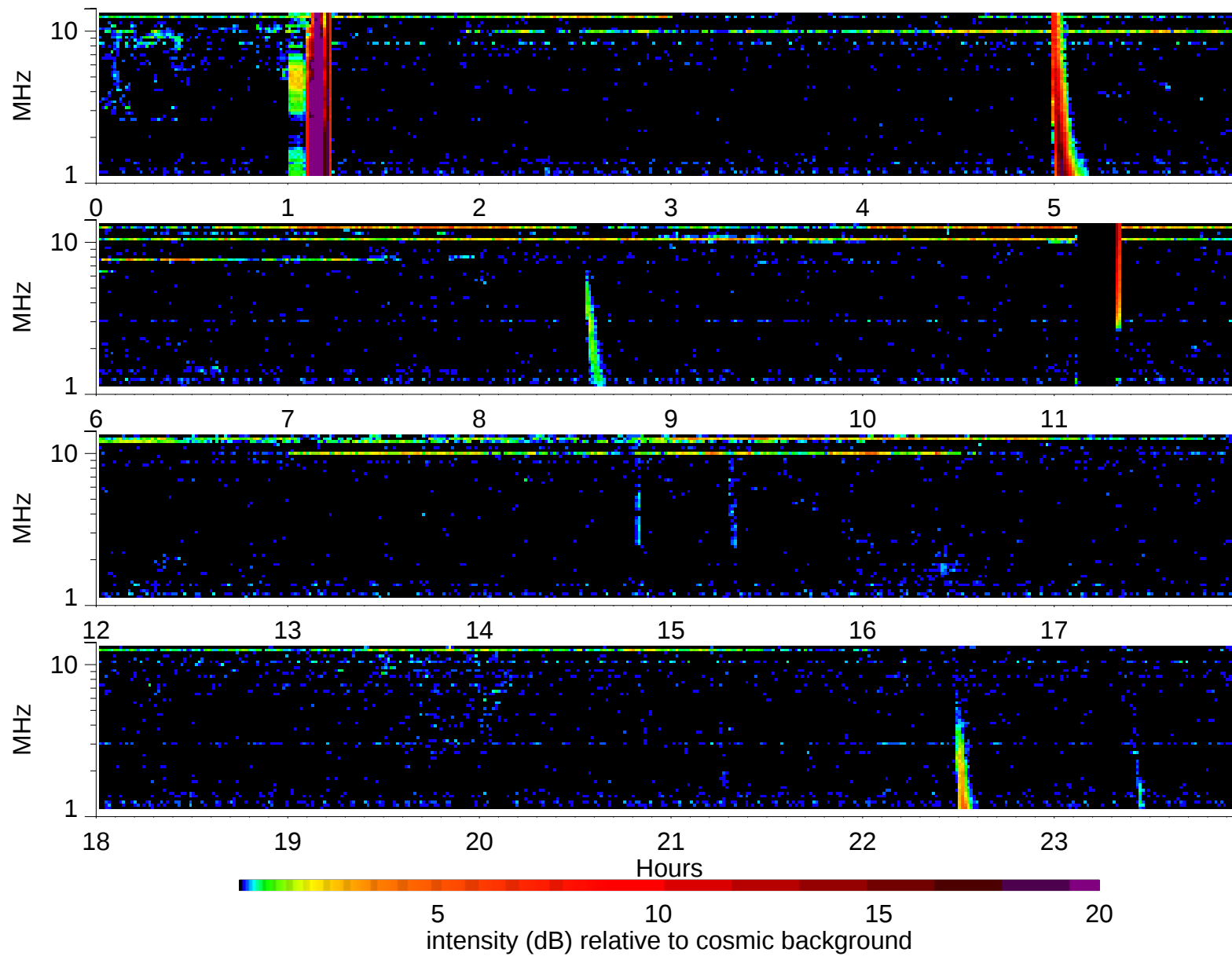
Wind Waves RAD2 receiver: 2005/7/1
