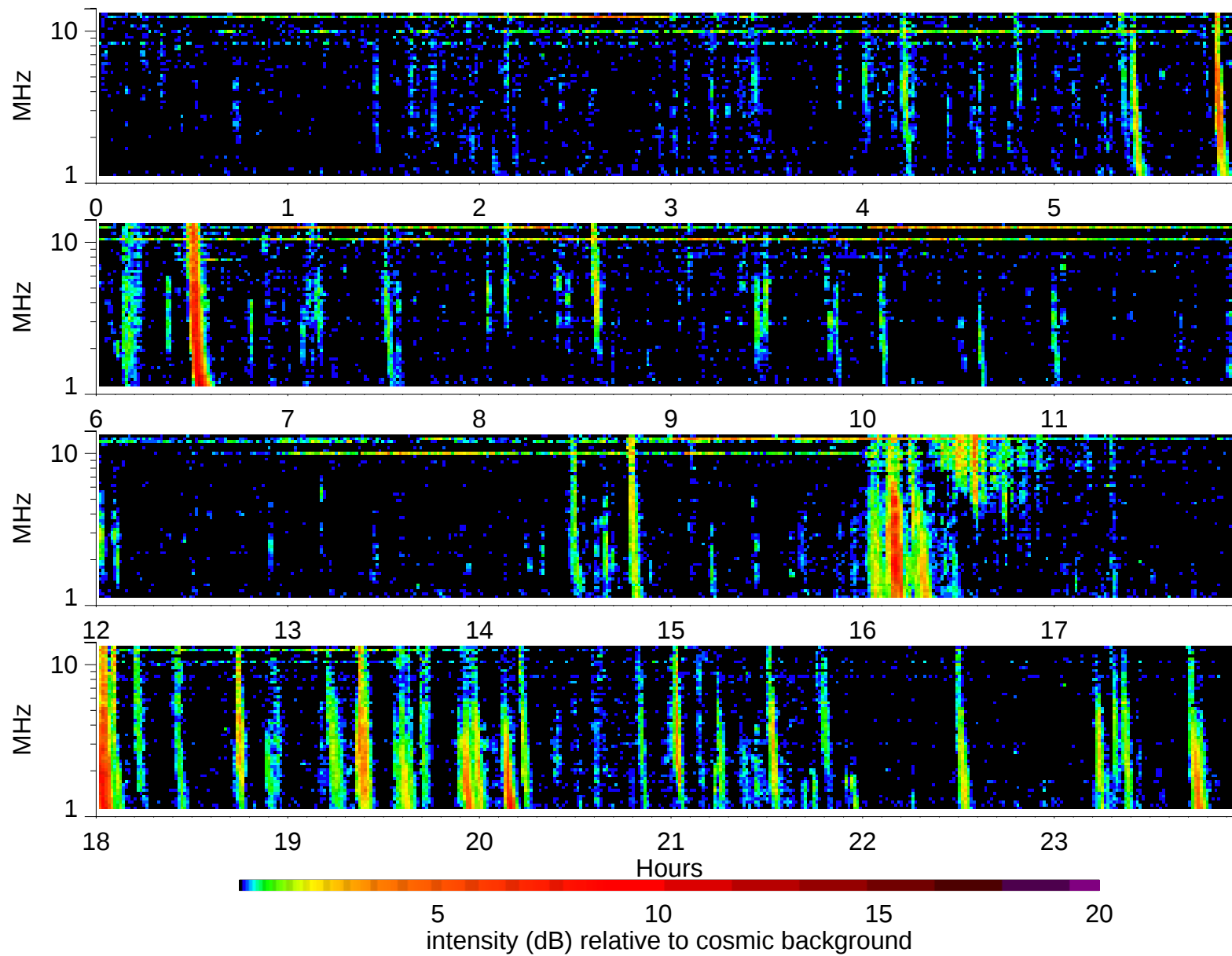
Wind Waves RAD2 receiver: 2005/7/8
