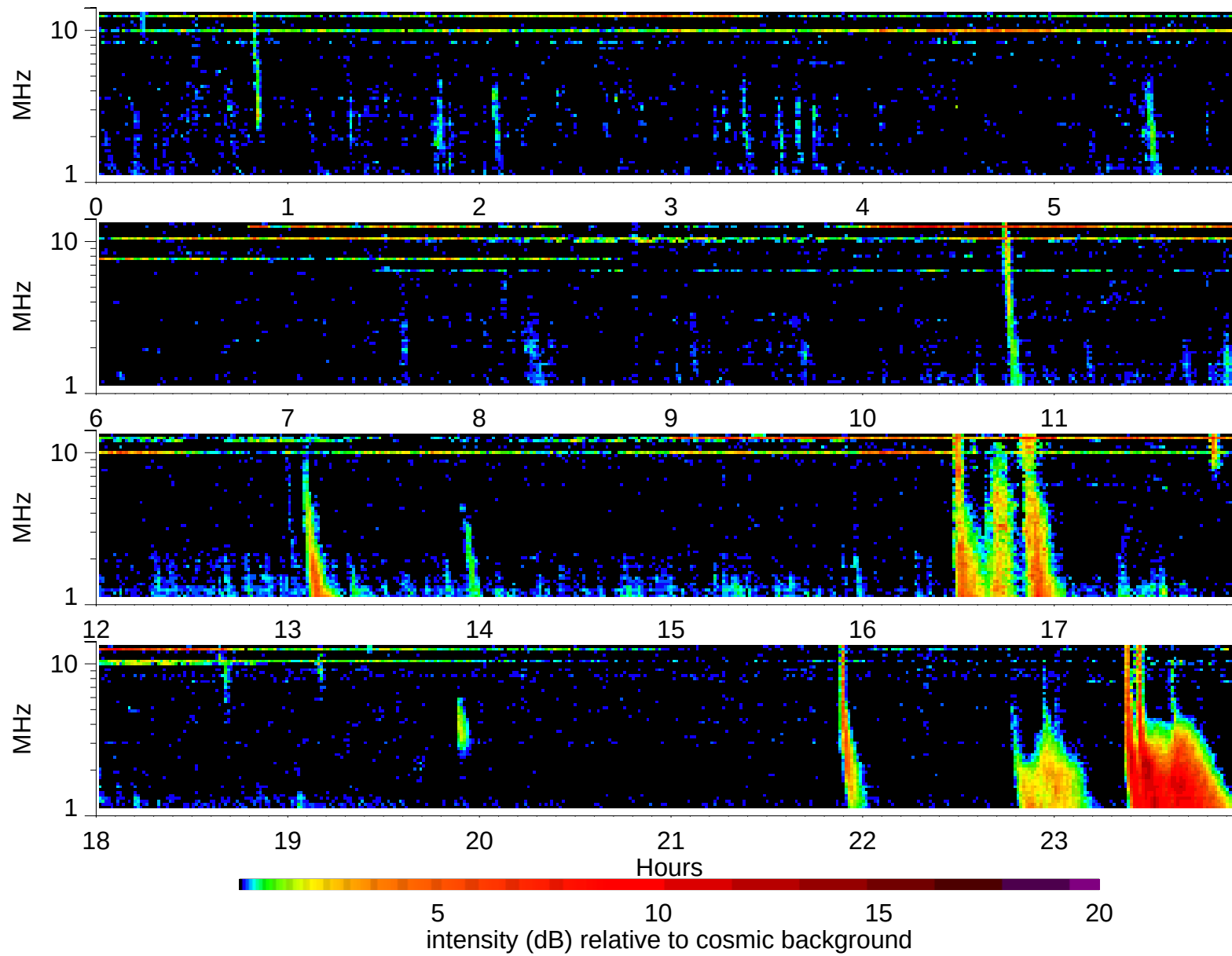
Wind Waves RAD2 receiver: 2005/7/12
