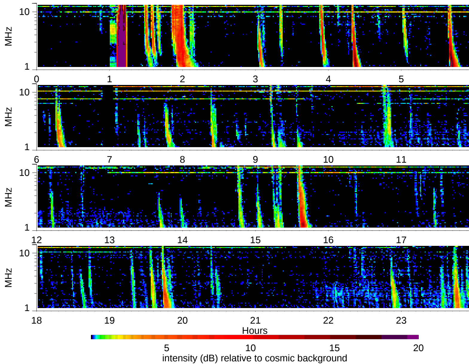
Wind Waves RAD2 receiver: 2005/7/15
