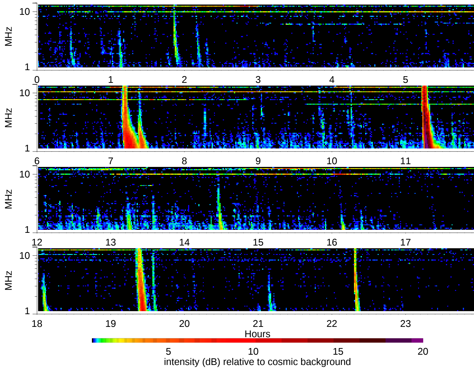
Wind Waves RAD2 receiver: 2005/7/16
