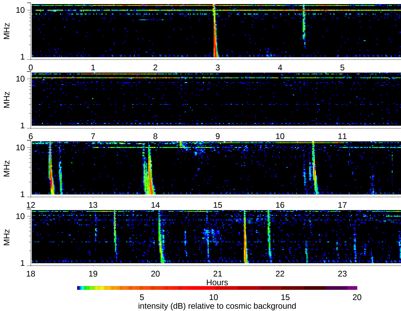
Wind Waves RAD2 receiver: 2005/8/1
