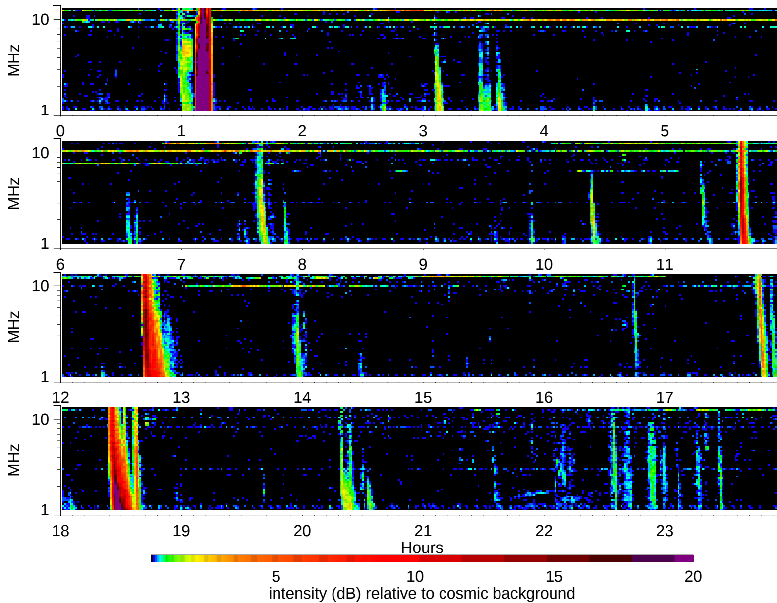
Wind Waves RAD2 receiver: 2005/8/2
