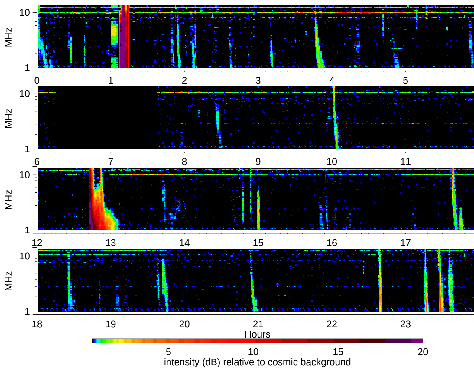
Wind Waves RAD2 receiver: 2005/8/4
