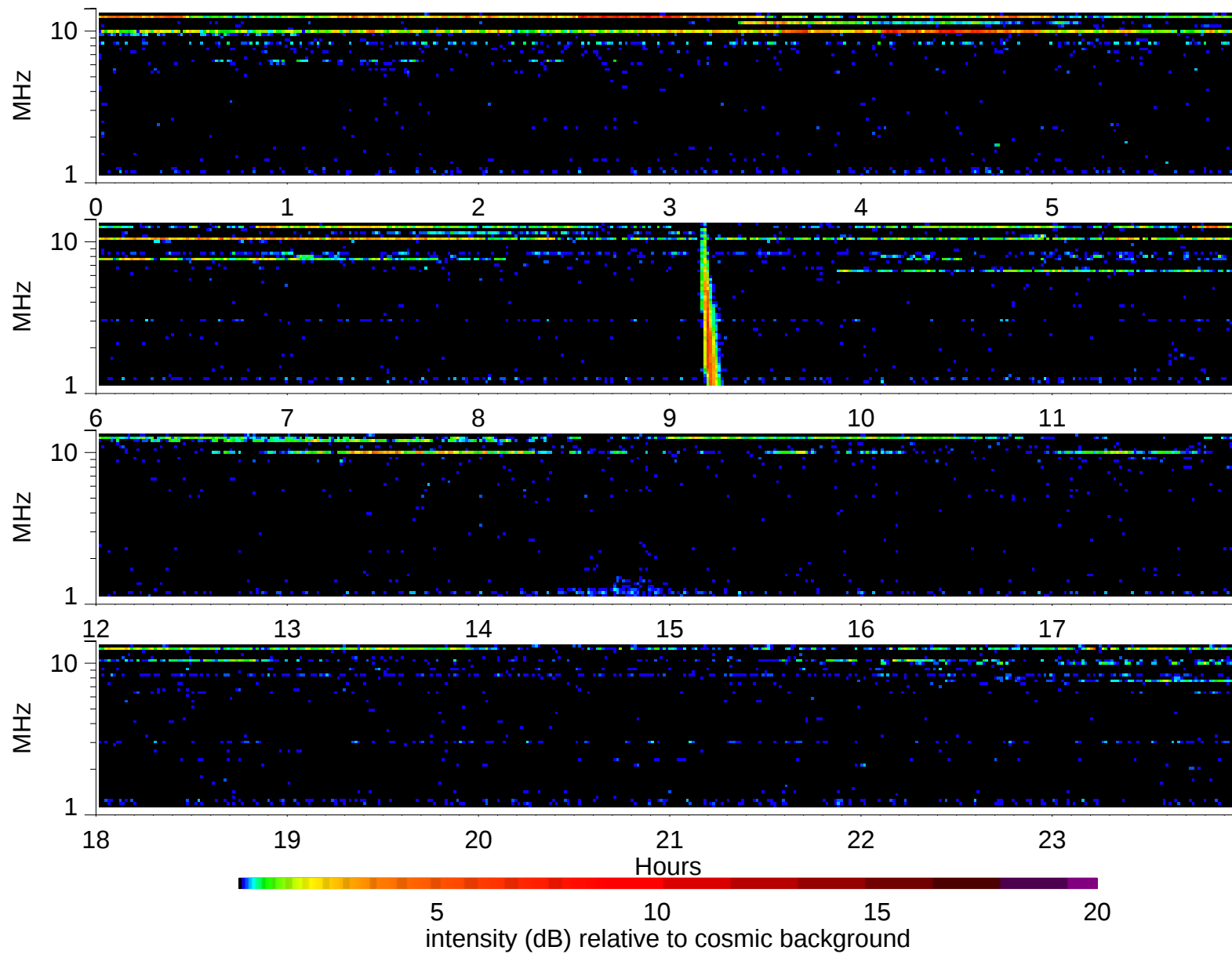
Wind Waves RAD2 receiver: 2005/8/11
