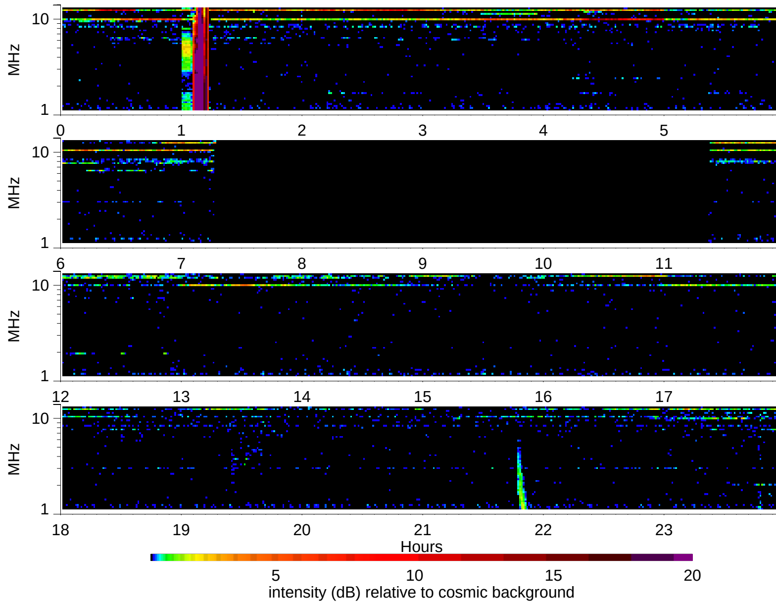
Wind Waves RAD2 receiver: 2005/8/16
